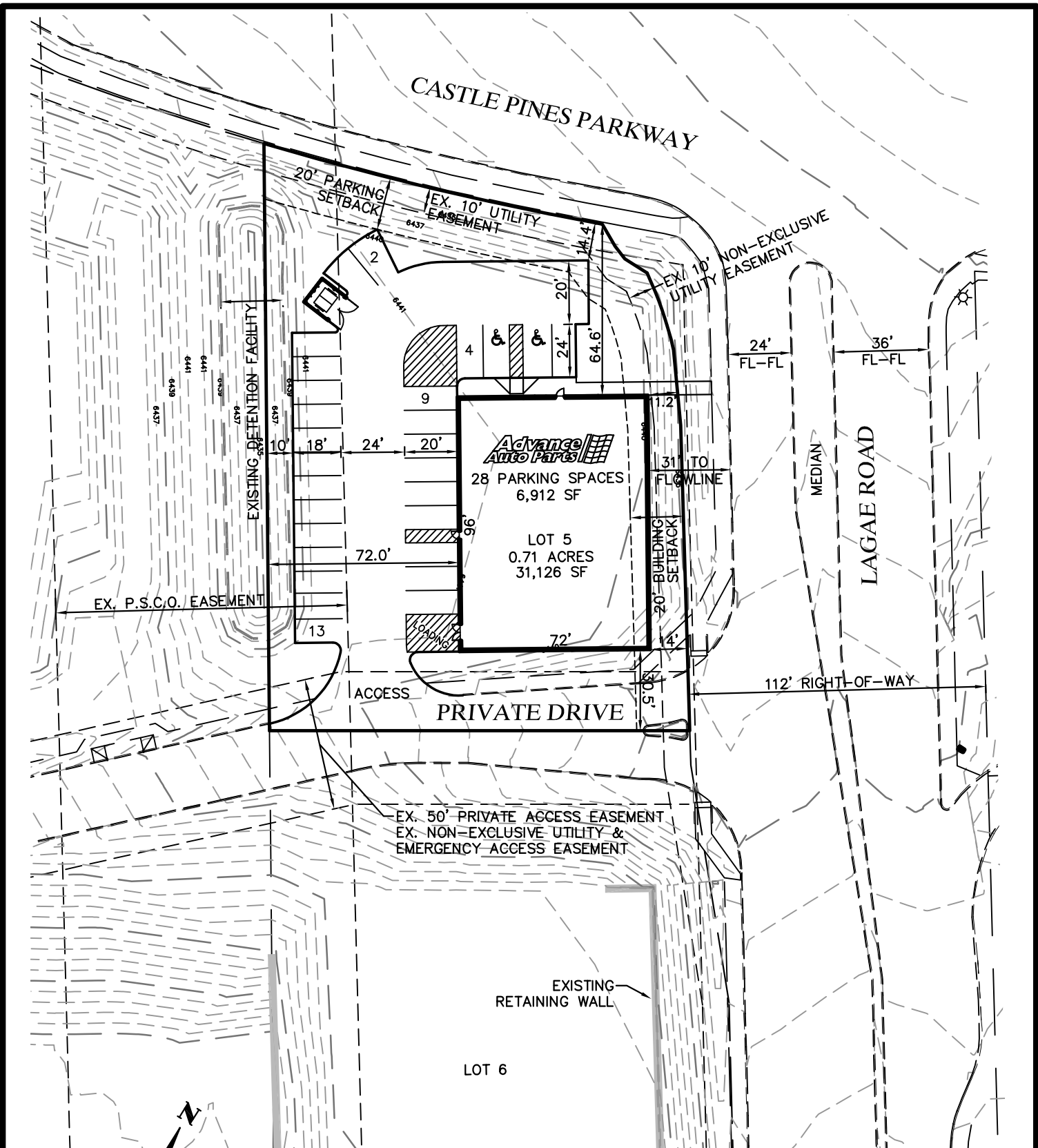
PROPOSED SITE PLAN LAYOUT (WITH TOPOGRAPHY)
